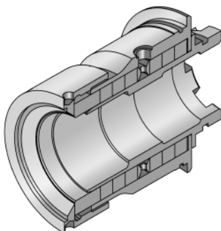
Shaft Seals Quenched, reversible mechanical seal as standard, optional Multiseal or Packing.
